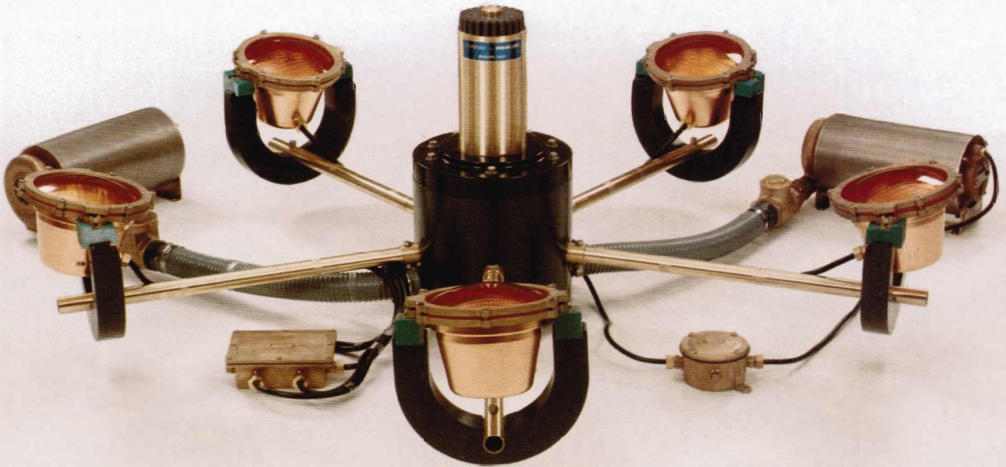
FIVE-LIGHT AQUAVATOR ASSEMBLY
